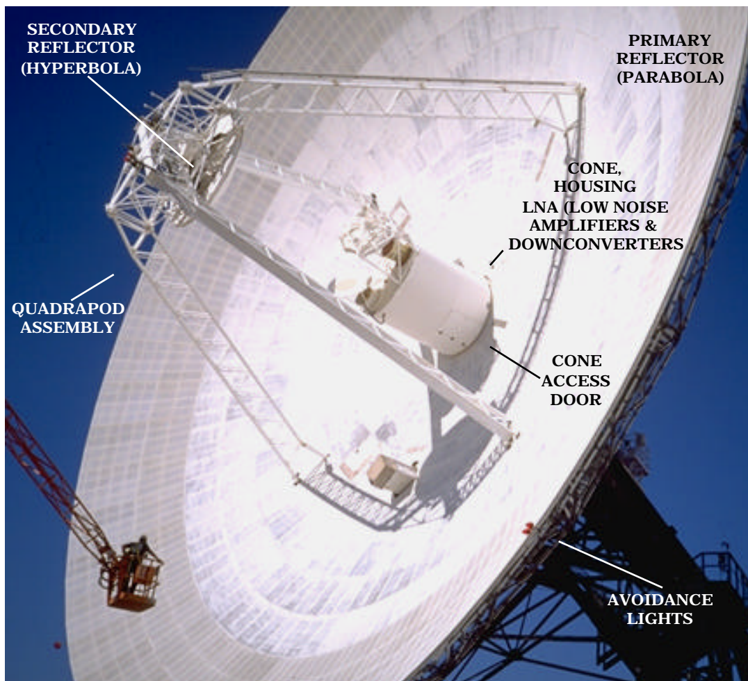
GAVRT ANTENNA REFLECTORS, CONE, AND QUADRAPOD
