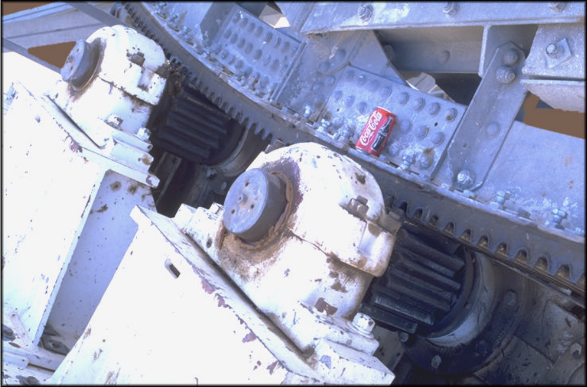
HOUR ANGLE BULL GEAR AND PINION GEARS
